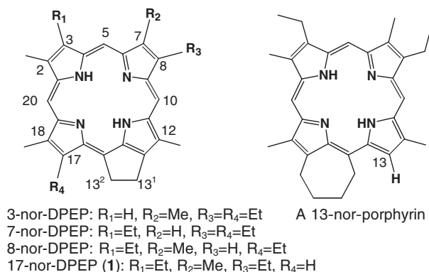
Figure 1. Sedimentary nor-porphyrins.
